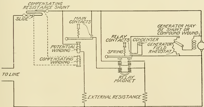
Fig. 17. Diagram for Tirrill Regulator Operating on Generator Field
